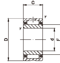
NA49,NA59,NA69( d \leq 30 ),NKI
