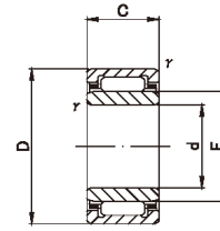
NKI(d ≤ 8)
